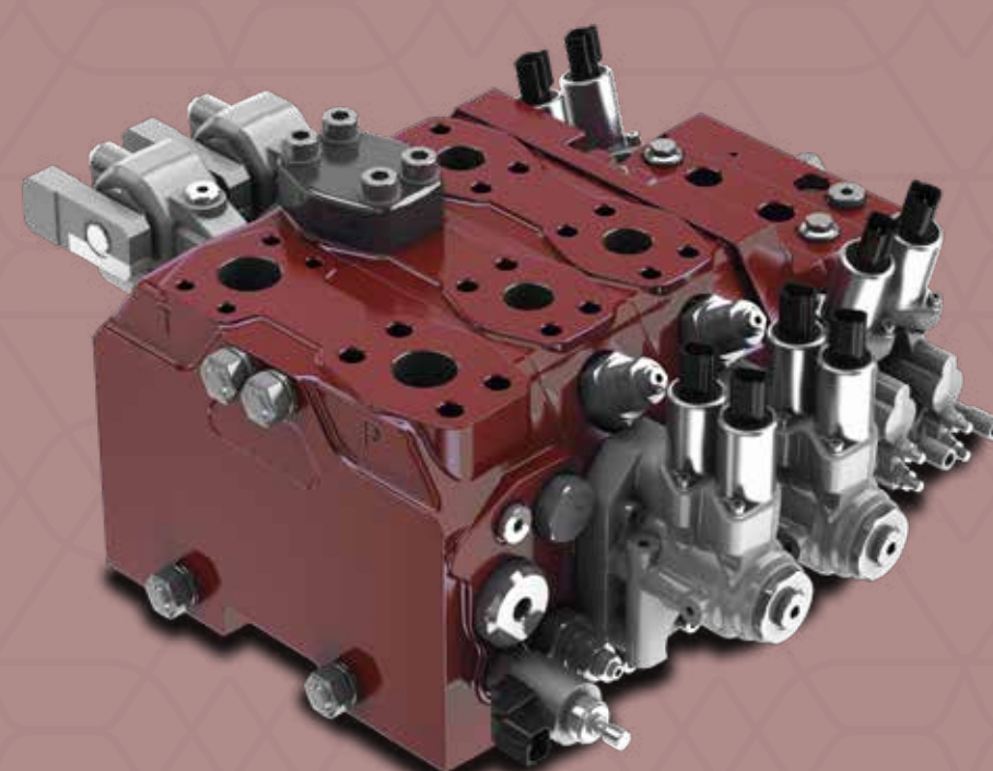
EX72+EX38 Full Flow Sharing directional control valves
