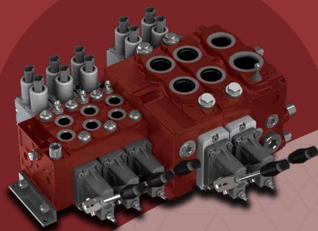
DPC200+DPC130 Load Sensing directional control valves
